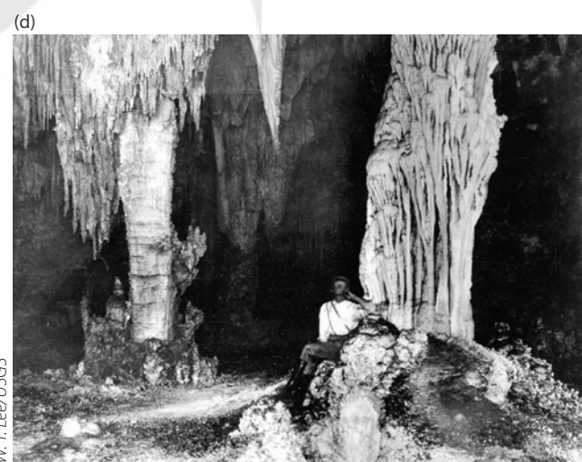
PHOTOGRAPH 4.15 Karst. Landscapes developed on limestone can be spectacular due to the effects of dissolution. (a) Touring watery passages of Mammoth Cave, Kentucky, by boat. The National Park Service discontinued tours such as this in the 1990s. [ Library of Congress, Prints & Photographs Division, Reproduction number LC-USZ62-47464 (b&w film copy neg.) ] (b) Sinkholes form as rock below collapses from dissolution. Here is a sinkhole in the Minnehakta limestone southeast of Boyd, Weston County, Wyoming, circa 1900. (c) Dramatic view of tower karst topography at river's edge, taken from a boat on a trip down the Li River south of Guilin, China. (d) Pillars of dripstone or flowstone deposited from calcium carbonate-saturated solutions at Carlsbad Caverns National Park, New Mexico.
