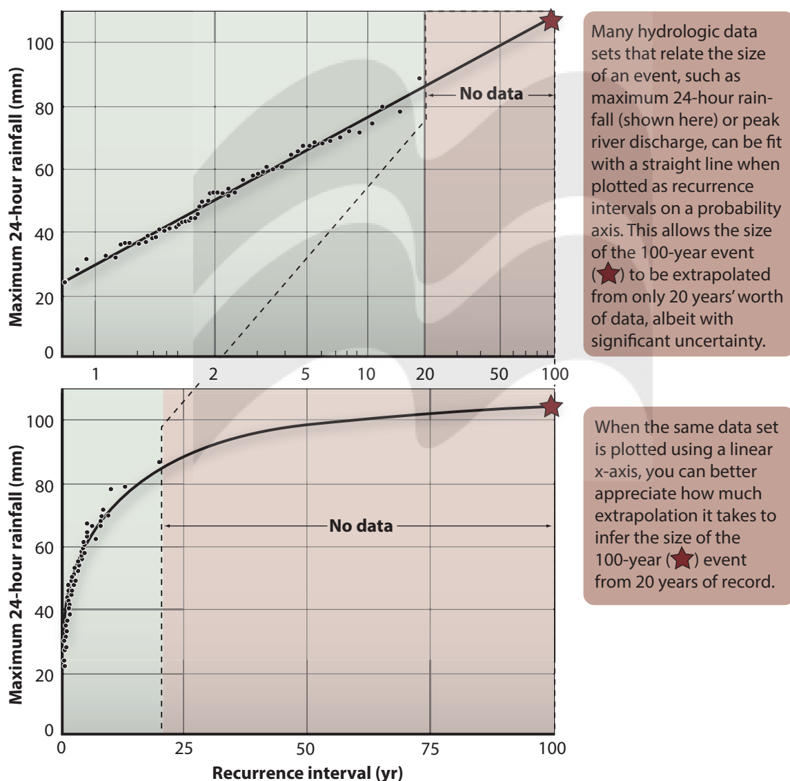
FIGURE 4.2 Precipitation Recurrence Interval with Extrapolation. Extreme hydrologic events are rare. Small events are common. Probability plots are a useful means of estimating how often an event of a particular size will recur. However, most periods of record are short, only a few decades, and extrapolation beyond the period of record is both commonplace and uncertain.
