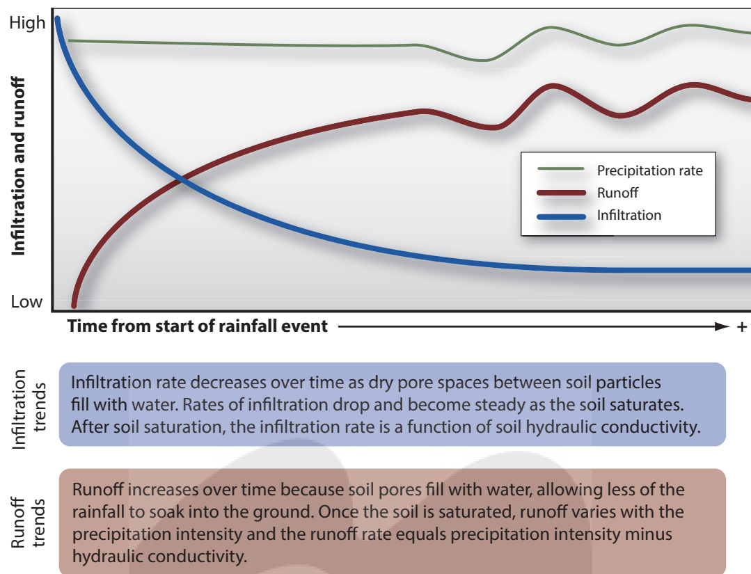
FIGURE 4.4 Infiltration and Runoff over Time. When rainfall begins, infiltration rates are high. As the ground saturates, infiltration rates drop off, and runoff begins as soon as the rate of precipitation exceeds the rate of infiltration.
