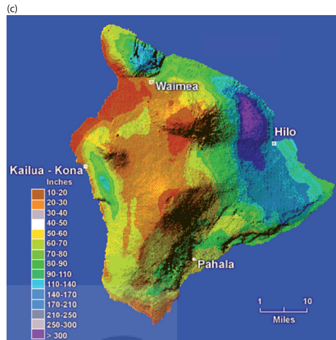
PHOTOGRAPH 4.14 Instrumentation Needed for Water Budgeting. (a) An early weather station (1880) with rain gauge on Pike's Peak, Colorado, at an elevation of ~ 4200 meters. (b) Dam and rectangular weir for measuring stream flow in the Los Angeles River in southern California, 1904. (c) Geography strongly controls the distribution of annual precipitation on the island of Hawaii. This map shows how wet the east side of the island is due to orographic lifting of moist tropical ocean air carried by northeasterly trade winds. The data are from the PRISM model, an algorithm that takes scarce observational data and combines these with terrain models to estimate the spatial variability of precipitation. [Oregon Climate Service / N.R.C.S. 4 × 4 km PRISM Model Grid. Based on 1961–90 annual precipitation data from NOAA Cooperative Stations. Hillshade relief derived from U.S. Geological Survey DEMs. Giambelluca, T.W., Q. Chen, A.G. Frazier, J.P. Price, Y.-L. Chen, P.-S. Chu, J.K. Eischeid, and D.M. Delaporte, 2013: Online Rainfall Atlas of Hawai'i. Bull. Amer. Meteor. Soc. 94, 313-316.]
