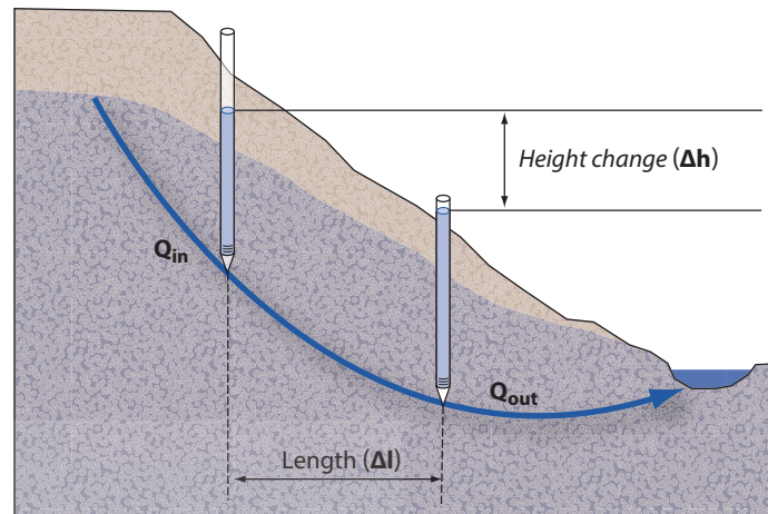
FIGURE 4.7 Darcy's Law. Darcy's Law explains the flux of groundwater as a function of energy gradient (change in head), the cross-sectional area through which the groundwater flows, and the ability of earth materials to pass water (their hydraulic conductivity).
